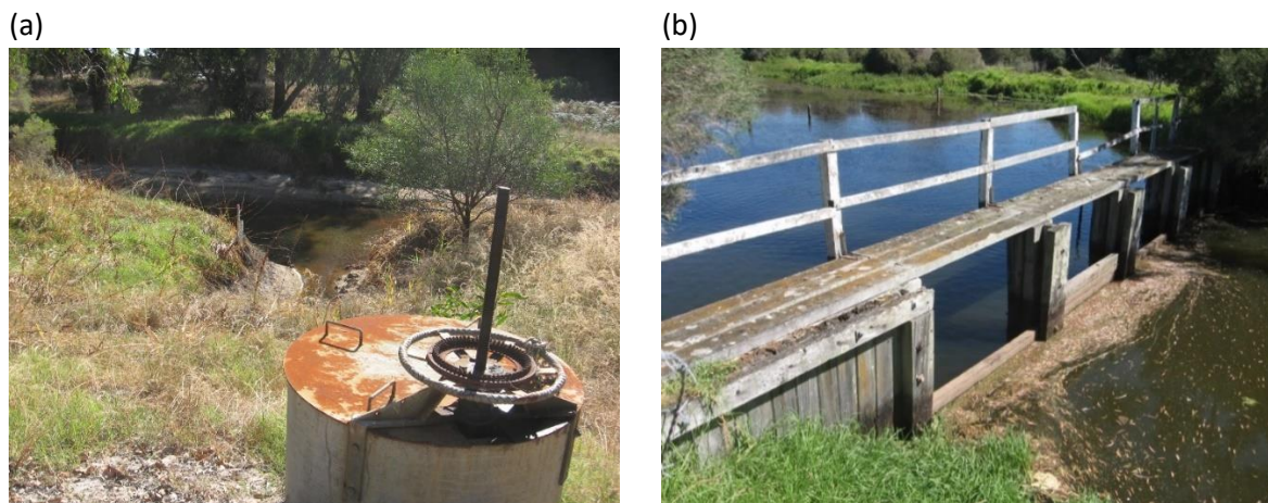
Figure 11. Flow management structures for the Lower Vasse River: (a) the valve controlling flow from the Vasse Diversion to the Lower Vasse River via a 900mm pipe; (b) the weir and removable boards at the Butter Factory.
